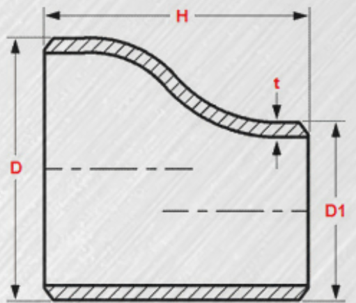
Reducer eccentric
