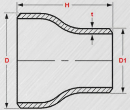
Reducer concentric
