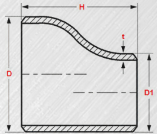
Reducer eccentric
